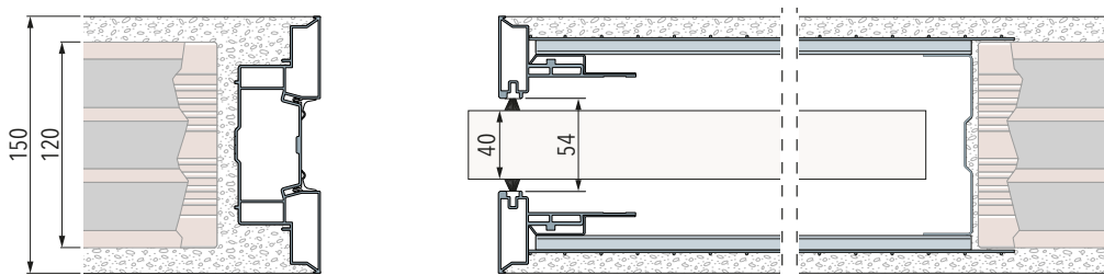
Pared acabada 150 mm - Ladrillo 120 mm
